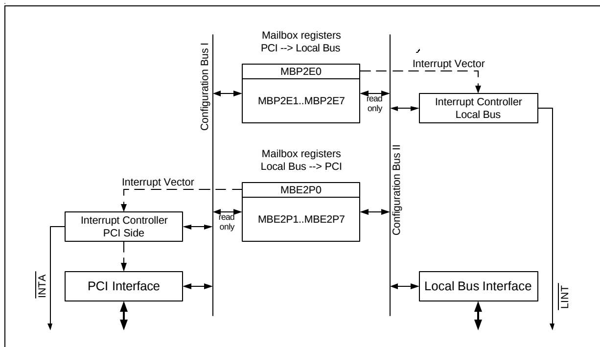
Figure 4-12 Mailbox Structure
