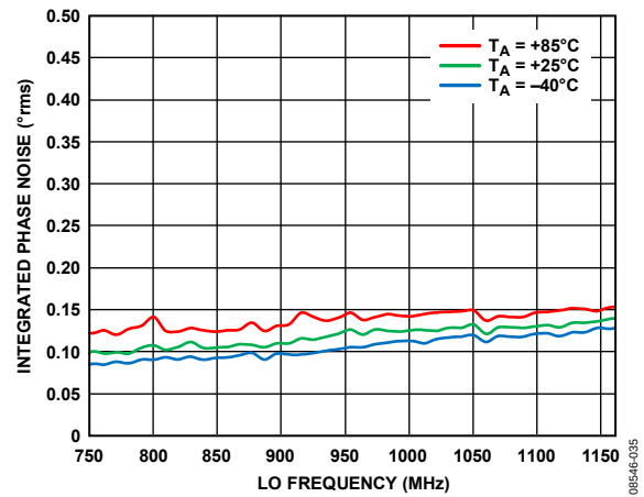
Figure 35. Integrated Phase Noise vs. LO Frequency
