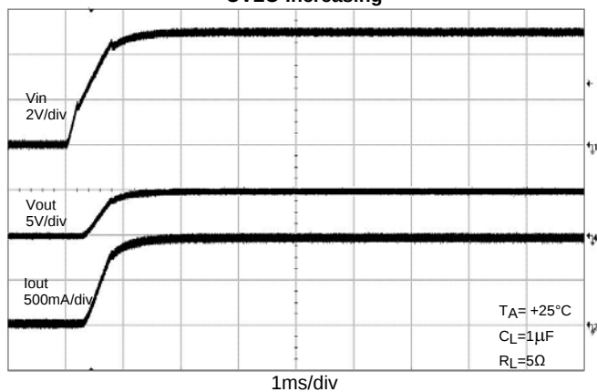
UVLO Increasing
