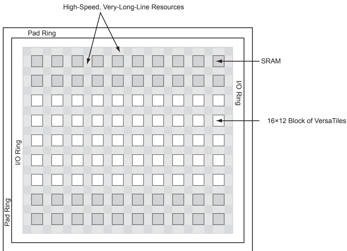
Figure 2-10 • Very-Long-Line Resources
