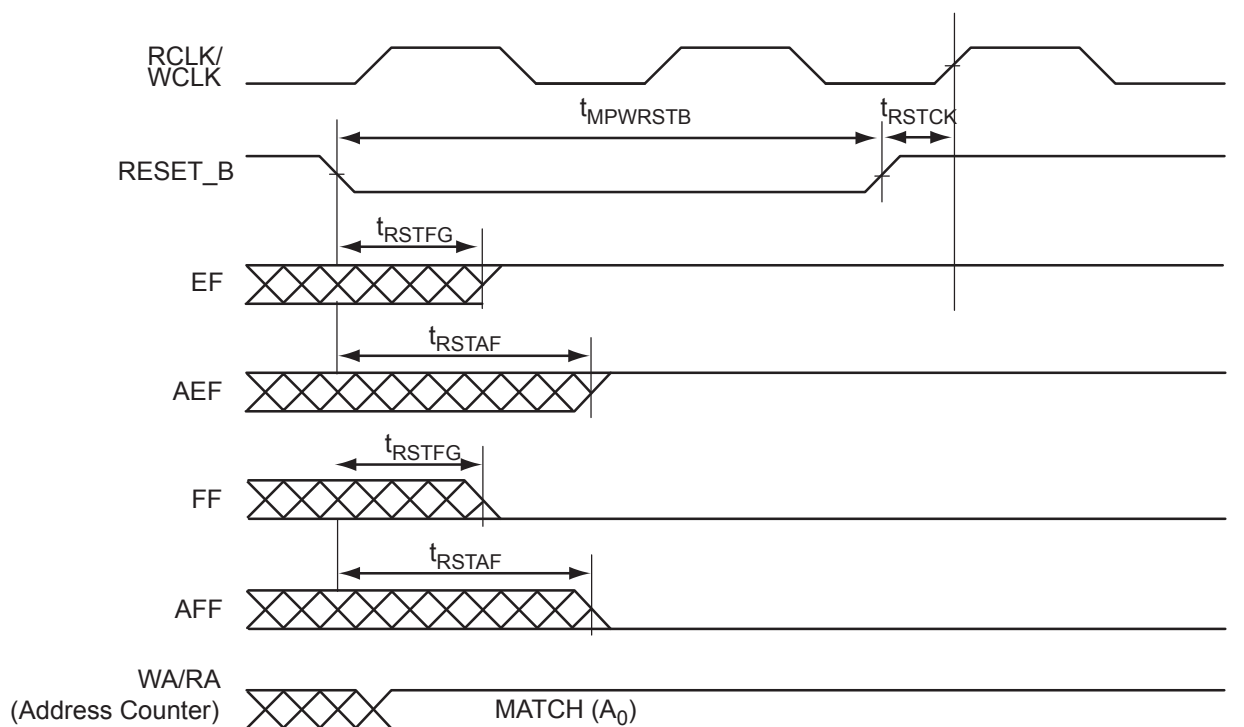
Figure 2-60 • FIFO Reset
