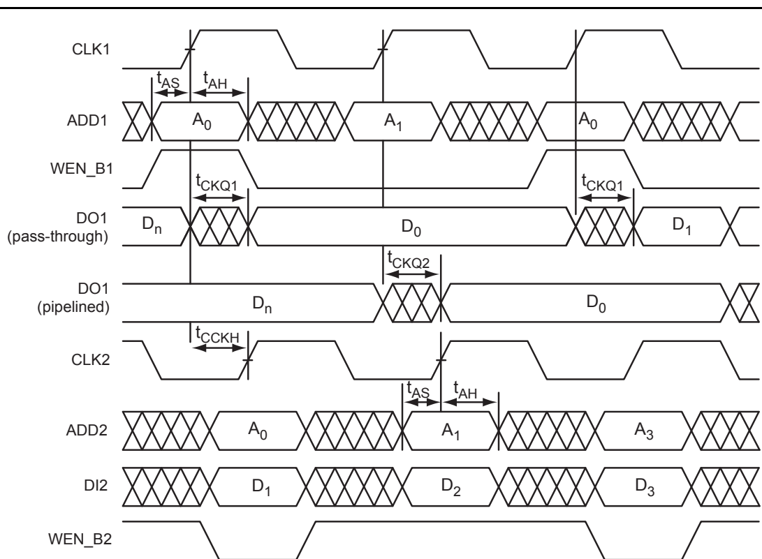
Figure 2-57 • Write Access After Read onto Same Address
