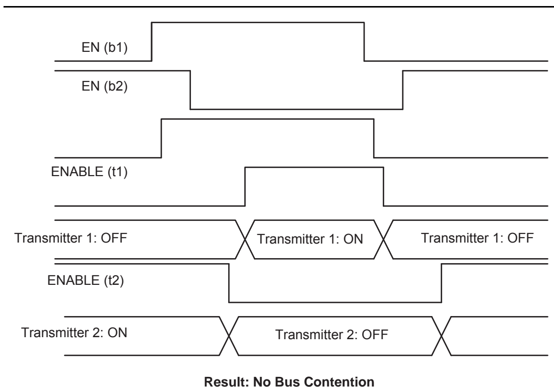
Figure 2-110 • Timing Diagram (with skew circuit selected)
