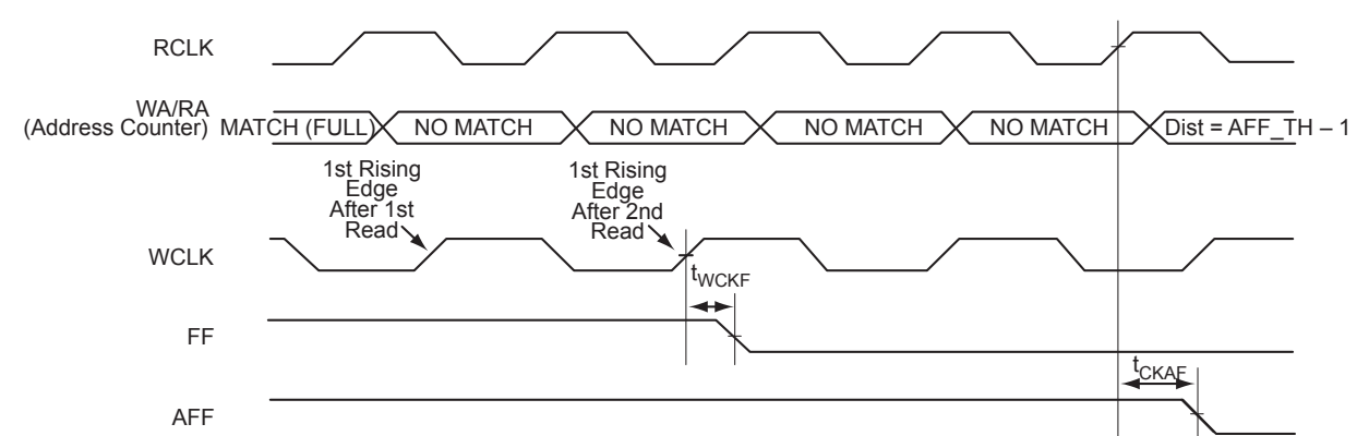
Figure 2-64 • FIFO FULL Flag and AFULL Flag Deassertion
