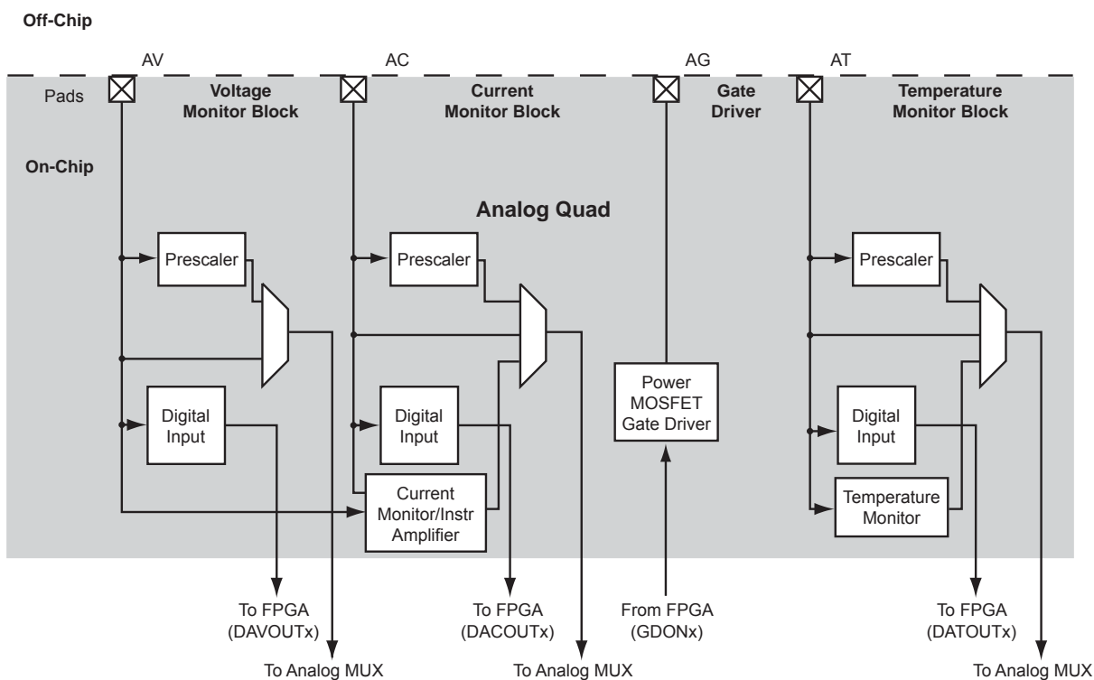
Figure 2-66 • Analog Quad
