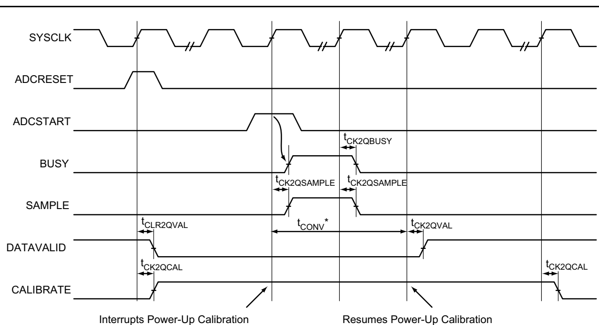
Figure 2-86 • Injected-Conversion Timing Diagram
