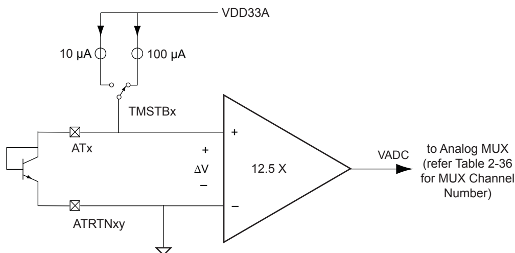
Figure 2-78 • Block Diagram for Temperature Monitor Circuit
