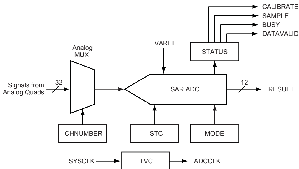
Figure 2-81 • ADC Simplified Block Diagram
