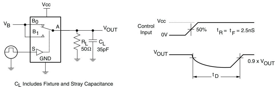
Figure 2. Break-Before-Make Timing
