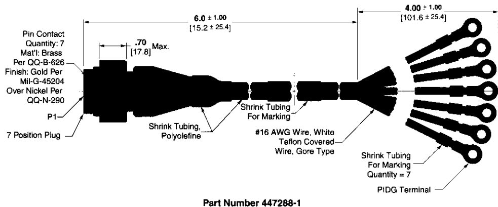
Part Number 447288-1
