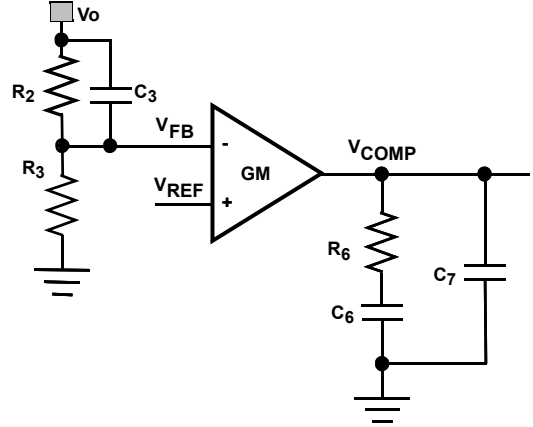
FIGURE 41. TYPE II COMPENSATOR
