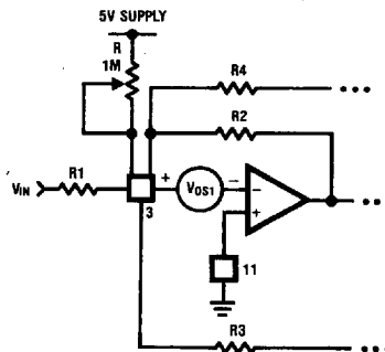
FIGURE 20. Method for Trimming V_{OS} , See Text, Section 3.4
