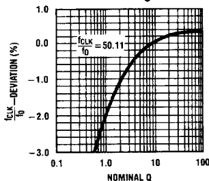
Deviation of \frac{f_{CLK}}{f_o} vs Nominal Q
