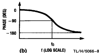
FIGURE 2. 2nd-Order Low-Pass Response
