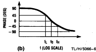
FIGURE 1. 2nd-Order Bandpass Response
