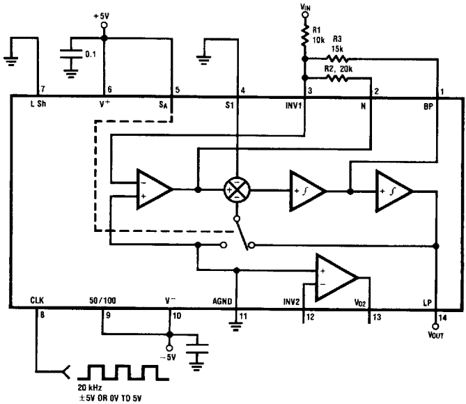
FIGURE 16. 2nd-Order Butterworth Low-Pass Filter of Design
