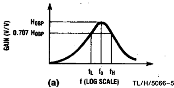
FIGURE 1. 2nd-Order Bandpass Response
