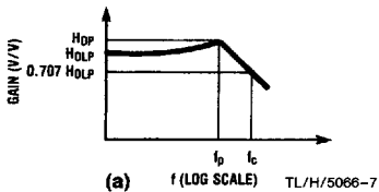
FIGURE 2. 2nd-Order Low-Pass Response
