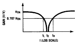
FIGURE 4. 2nd-Order Notch Response
