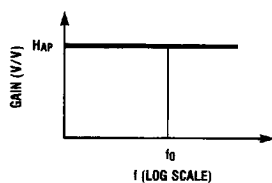
FIGURE 5. 2nd-Order All-Pass Response
