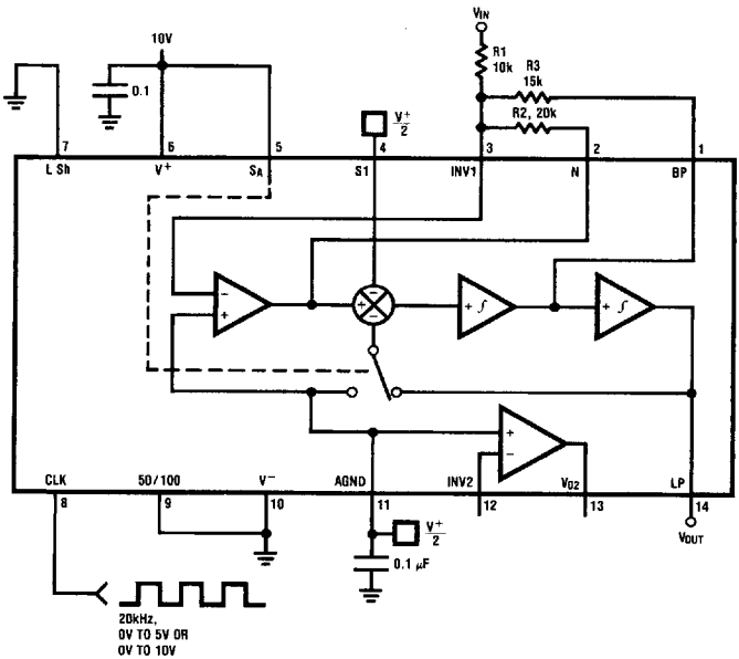
FIGURE 17. Butterworth Low-Pass Circuit of Example, but Designed for Single-Supply Operation
