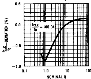
Deviation of \frac{f_{CLK}}{f_o} vs Nominal Q
