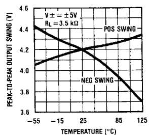
OPAMP Output Voltage Swing vs Temperature
