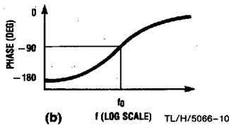
FIGURE 3. 2nd-Order High-Pass Response
