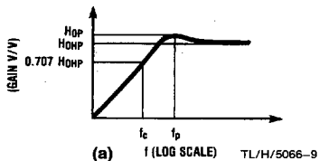
FIGURE 3. 2nd-Order High-Pass Response
