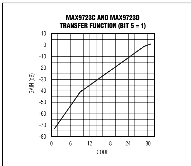
Figure 9. MAX9723C/MAX9723D Transfer Function with Bit 5 = 1
