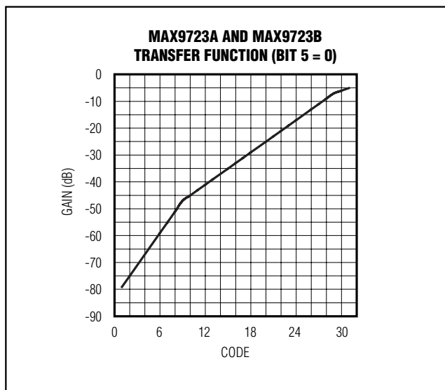
Figure 8. MAX9723A/MAX9723B Transfer Function with Bit 5 = 0
