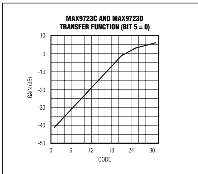
Figure 10. MAX9723C/MAX9723D Transfer Function with Bit 5 = 0
