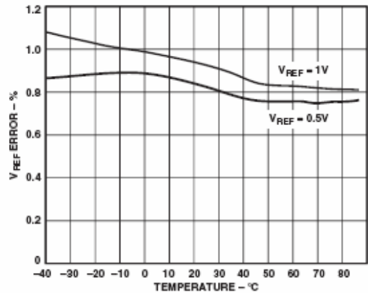
Figure 10. Typical V_{REF} Drift
