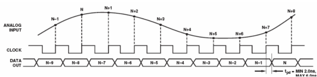
Figure 2. Timing Diagram
