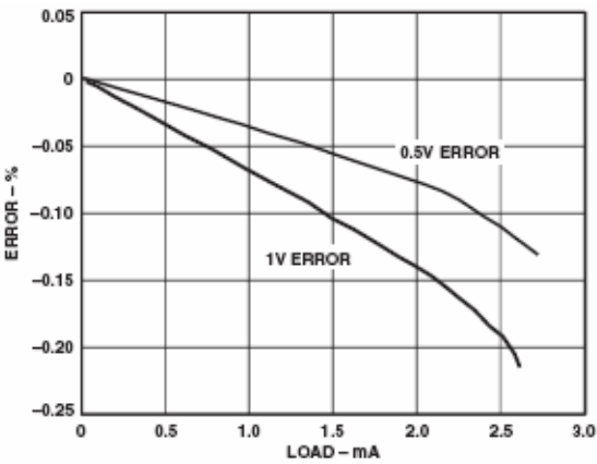
Figure 11. V_{REF} Accuracy vs. Load
