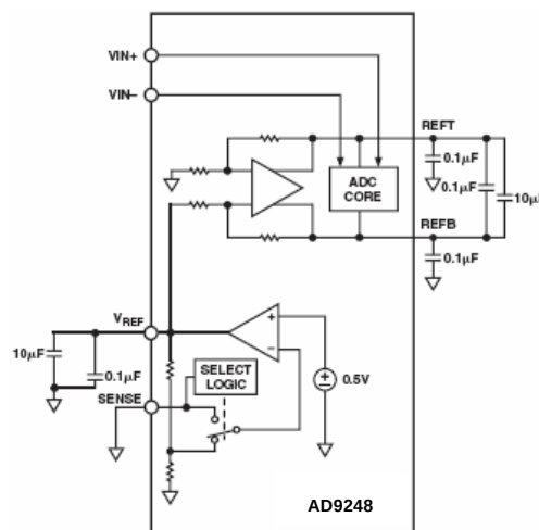
Figure 8. Internal Reference Configuration
