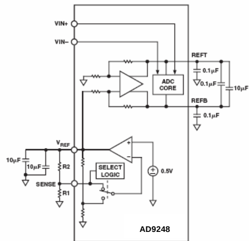
Figure 9. Programmable Reference Configuration
