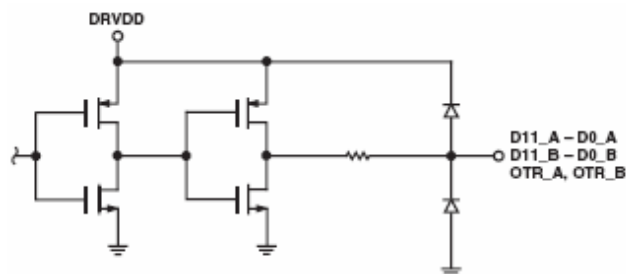
Figure 3. Equivalent Digital Output Circuit
