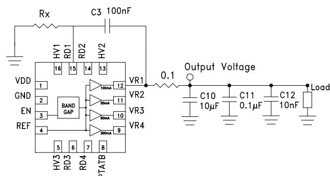
Figure 16. Recommended HMC1060LP3E configuration for supplying output voltage values greater than default. [4]
