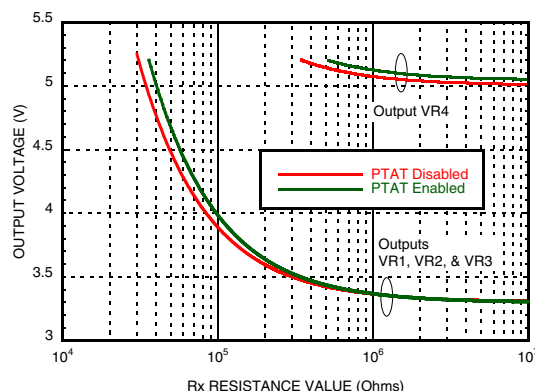
Figure 17. HMC1060LP3E output voltage as a function of resistance Rx for each output at 27°C. [5]
