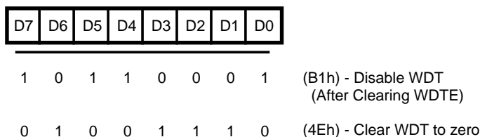
Figure 93. Watch-Dog Timer Command Register
