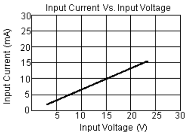
Characteristic Curves
