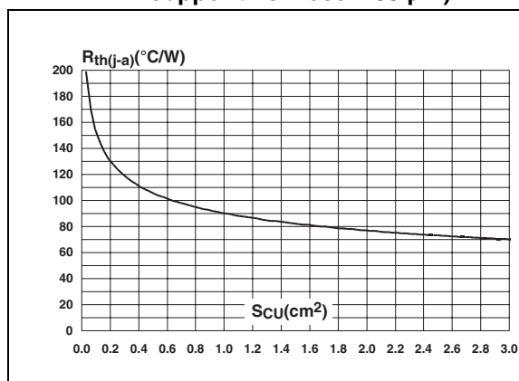
Figure 8. Thermal resistance junction to ambient versus copper surface under each lead (printed circuit board FR4, copper thickness = 35\text{ }\mu\text{m} )
