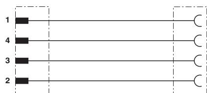
Contact assignment of M8 plugs / M12 sockets
