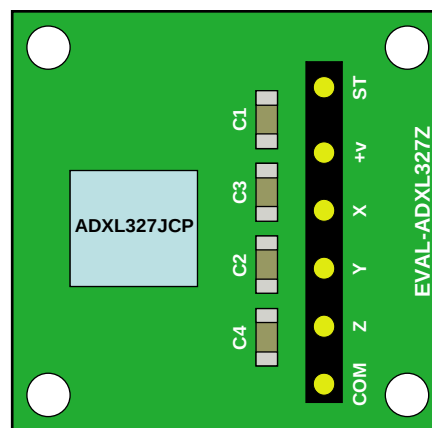
Figure 2. Physical Layout
