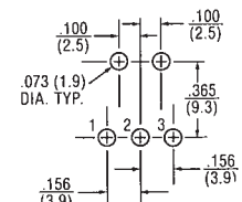
Mounting Information
