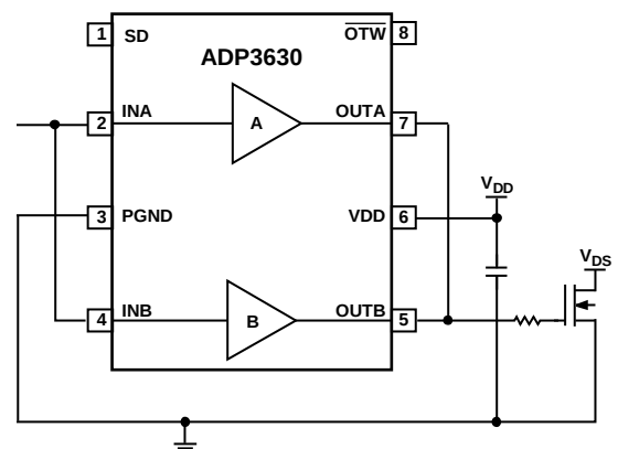
Figure 25. Parallel Operation
