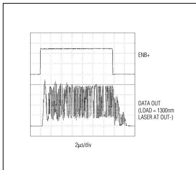
Figure 3. Enable/Disable Operation
