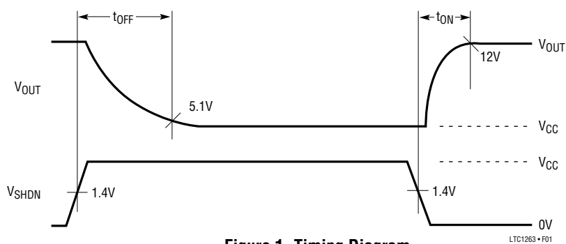
Figure 1. Timing Diagram
