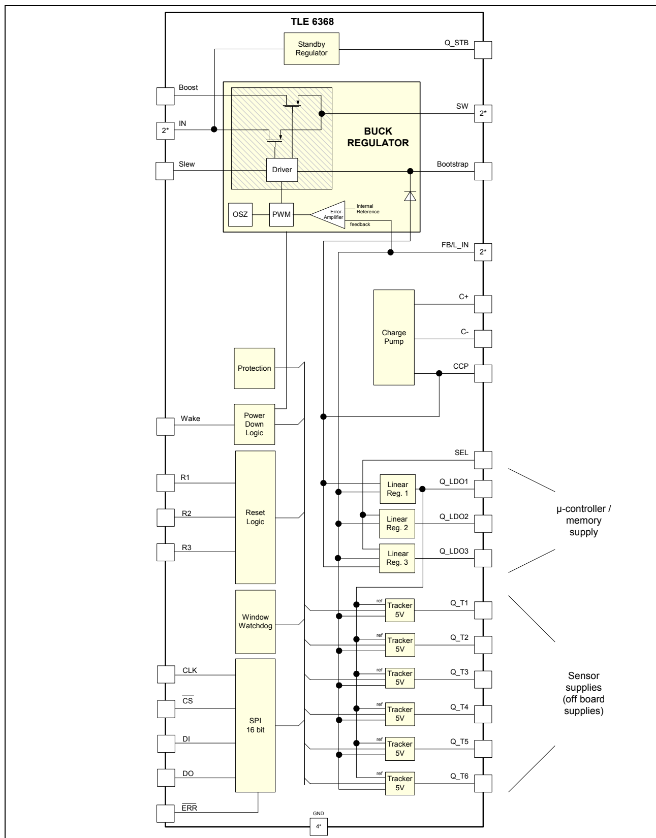
Figure 2 Block Diagram
