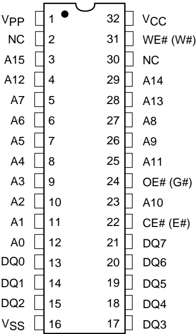
PDIP
