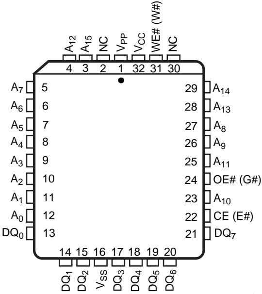
PLCC
