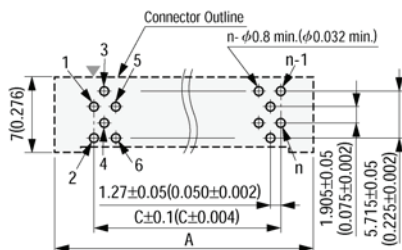
Printed Circuit Board Layout (Component Side View) Printed Circuit Board Layout (Component Side View)
