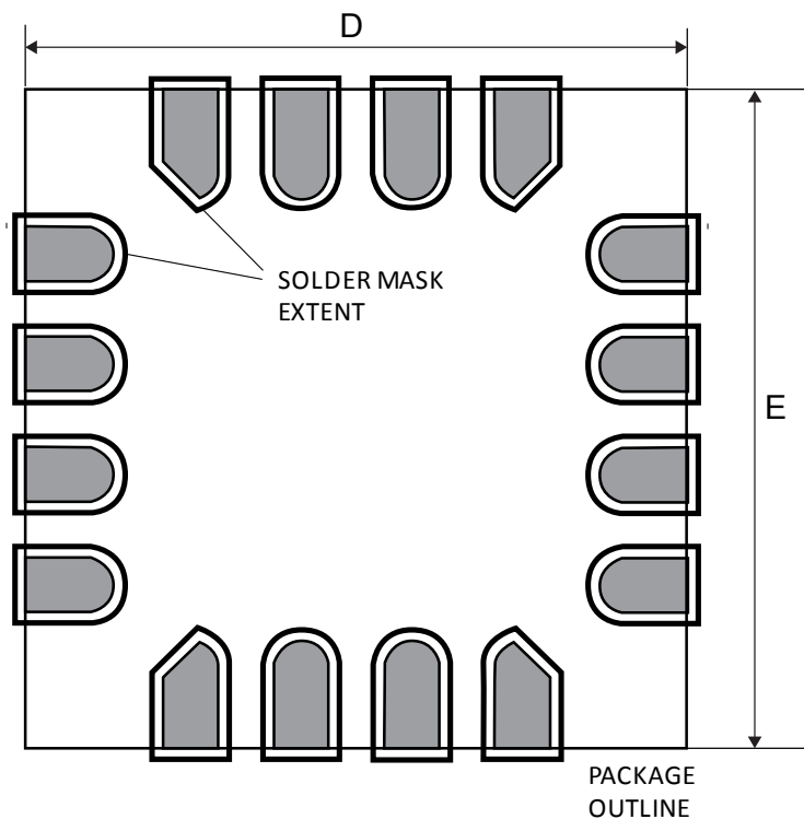
Individually Outlined Pads – Solder Mask
