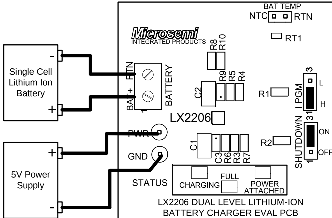
Figure 3 – LX2206 Typical Test Hookup
