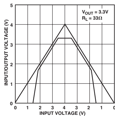
TPC 8. Power-Up/Power-Down
