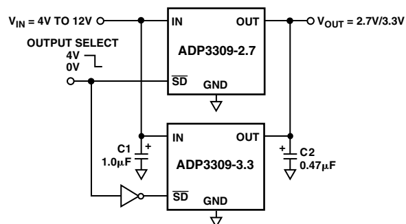
Figure 3. Crossover Switch
