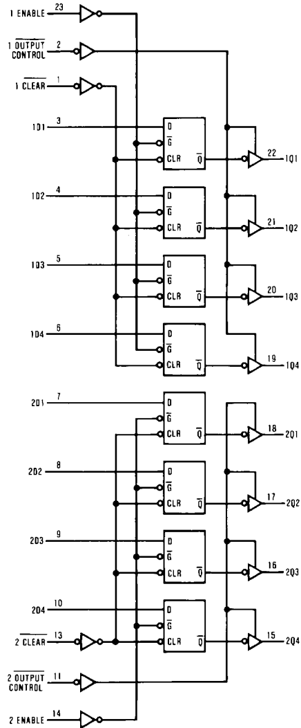
Logic Diagram
