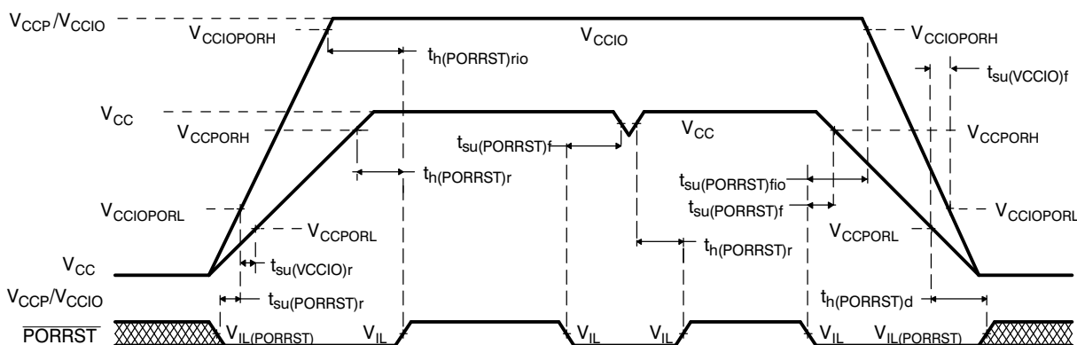
Figure 9. \overline{PORRST} Timing Diagram
