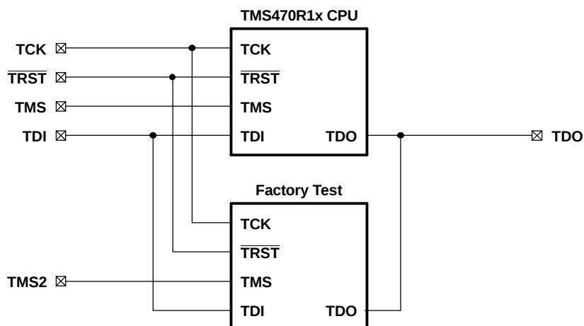
Figure 2. JTAG Interface
