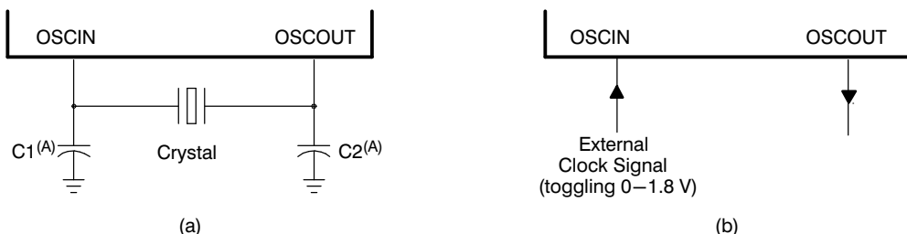
Figure 6. Crystal/Clock Connection
