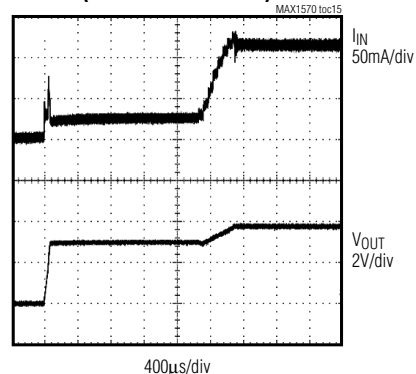
STARTUP RESPONSE ( V_{IN} = 3.3V ) (5 LEDs AT 15mA/LED)
