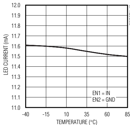
LED CURRENT vs. TEMPERATURE ( V_{IN} = 3.3V , R_{SET} = 7.5k\Omega )
