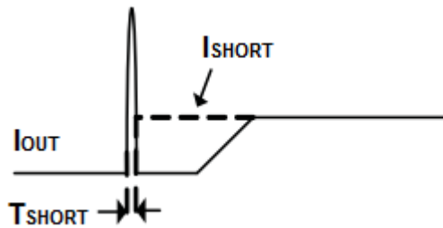
Figure 2. Response Time to Short Circuit Waveform
