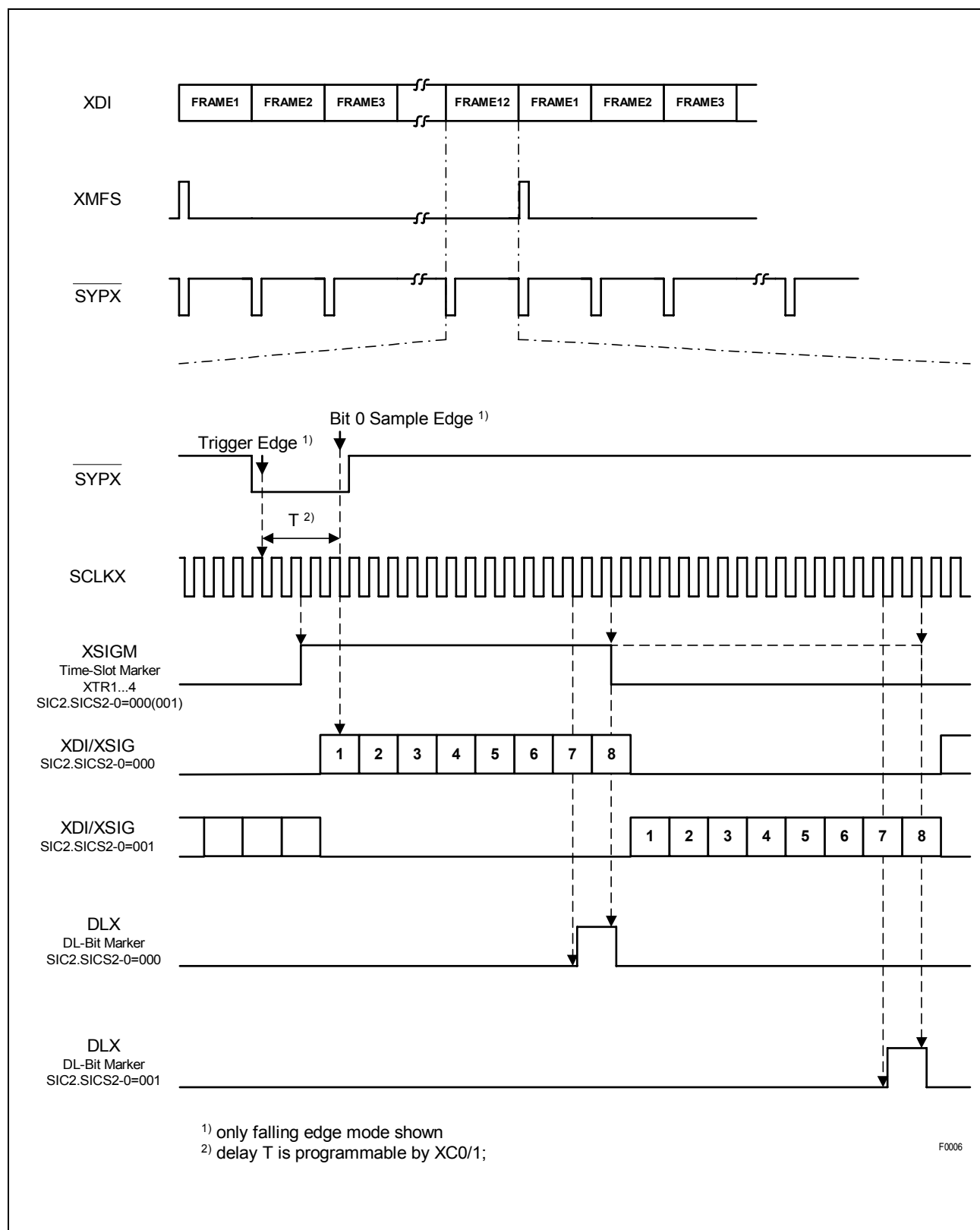
Figure 69 Transmit System Clocking: 8.192 MHz/4.096 Mbit/s (T1/J1)
