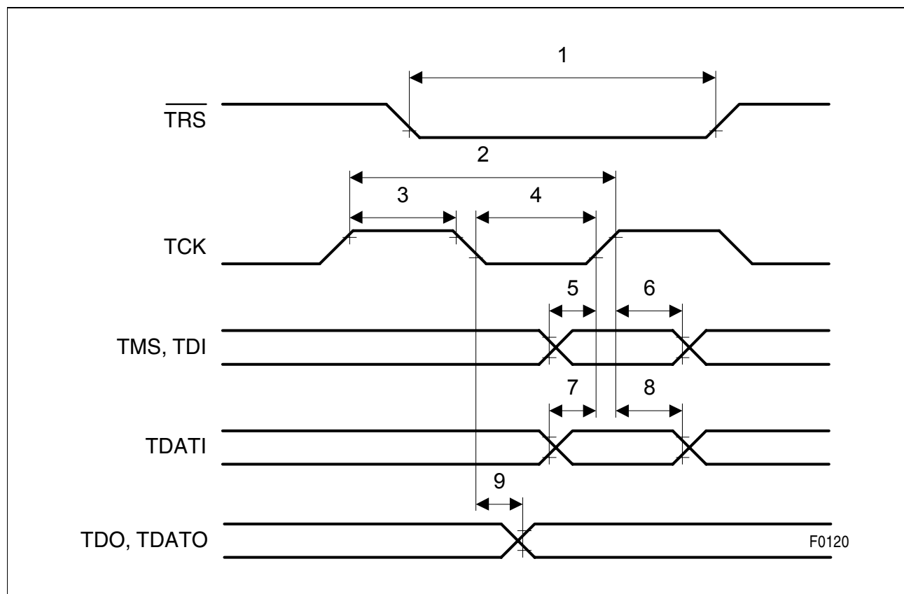
Figure 87 JTAG Boundary Scan Timing
