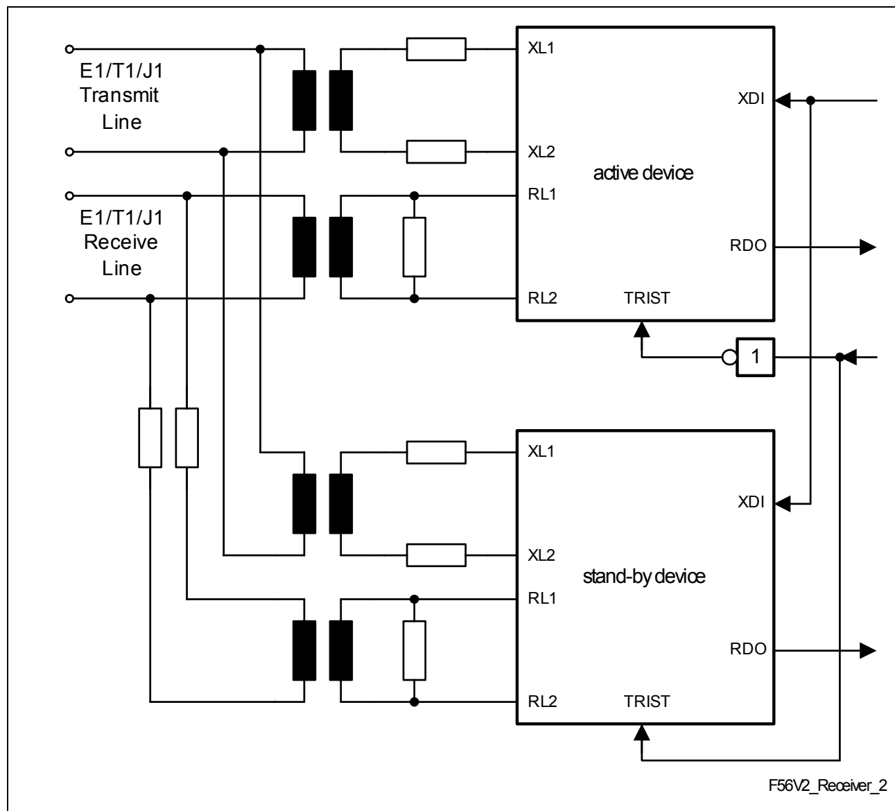
Figure 19 Short Haul Protection Switching Application (E1)
