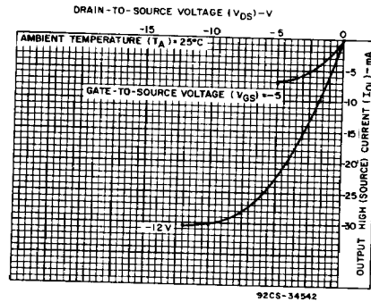
Fig. 10 - Minimum output high (source) current characteristics - TTL to CMOS.
