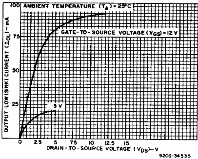
Fig. 3 - Typical N-Channel output low (sink) current characteristics - CMOS to TTL.
