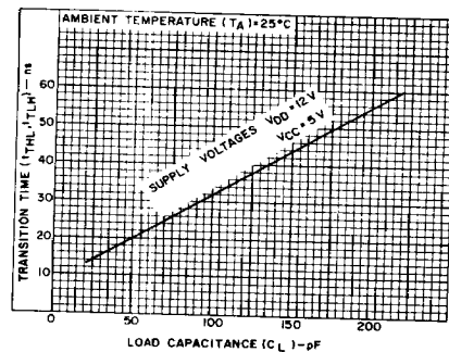
Fig. 12 - Typical transition time as a function of load capacitance CMOS-to-TTL or TTL-to-CMOS.
