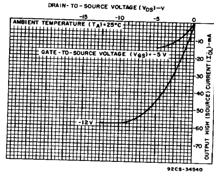
Fig. 8 - Typical output high (source) current characteristics - TTL to CMOS.
