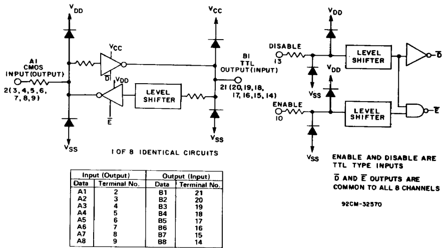
Fig. 1 - Functional block diagram.
