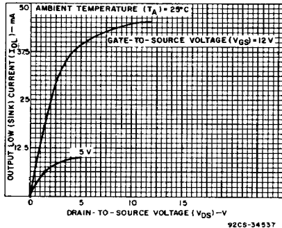
Fig. 5 - Minimum N-Channel output low (sink) current characteristics - CMOS
