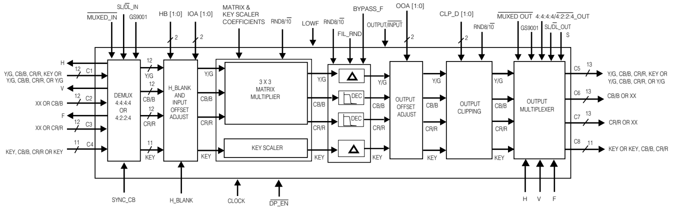
Fig. 5d Functionality of GF9105A Processing Core when \text{INT}/\overline{\text{DEC}} = 0 , \text{HVF\_OUT} = 1
