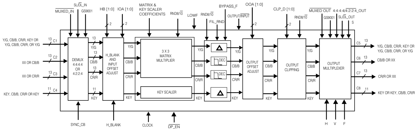
Fig. 5b Functionality of GF9105A Processing Core when \text{INT}/\overline{\text{DEC}} = 0 , \text{HVF\_OUT} = 0
