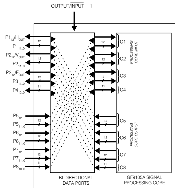
Fig. 4d Functional Block Diagram of GF9105A ( \text{OUTPUT}/\overline{\text{INPUT}} = 1 , \text{HVF\_OUT} = 1 )
