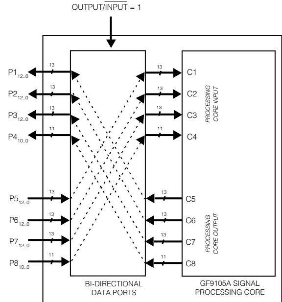
Fig. 4b Functional Block Diagram of GF9105A ( \text{OUTPUT}/\overline{\text{INPUT}} = 1 , \text{HVF\_OUT} = 0 )
