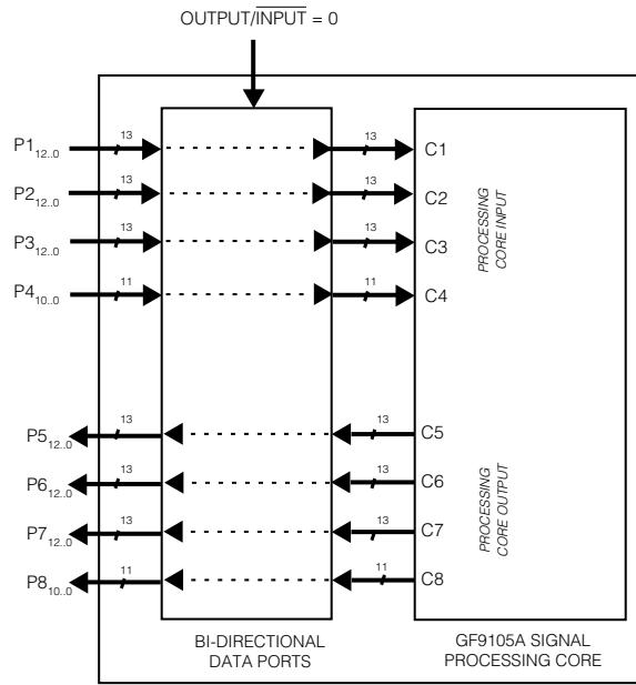
Fig. 4a Functional Block Diagram of GF9105A ( \text{OUTPUT}/\overline{\text{INPUT}} = 0 , \text{HVF\_OUT} = 0 )
