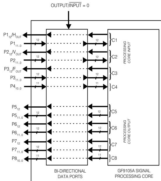
Fig. 4c Functional Block Diagram of GF9105A ( \text{OUTPUT}/\overline{\text{INPUT}} = 0 , \text{HVF\_OUT} = 1 )
