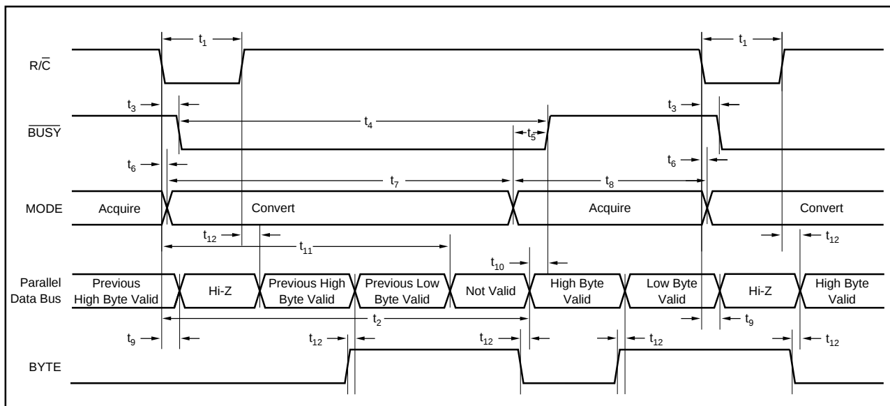
FIGURE 2. Conversion Timing with Parallel Output ( \overline{\text{CS}} LOW).
