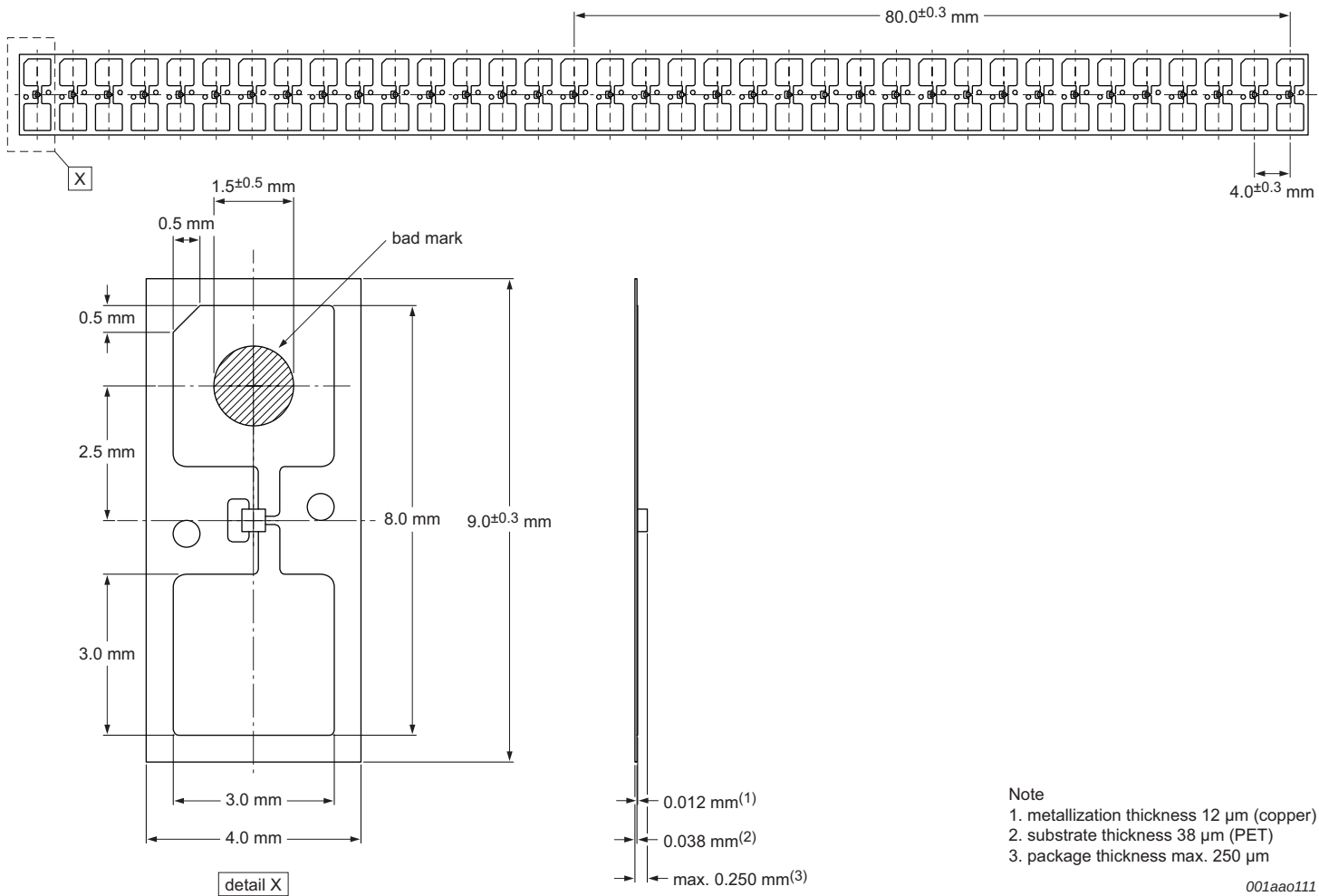
Fig 9. Package FCS2, SOT1040AA1, 12 μm Cu metallization
