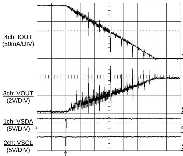
Waveform when it drives from Full code to 0
