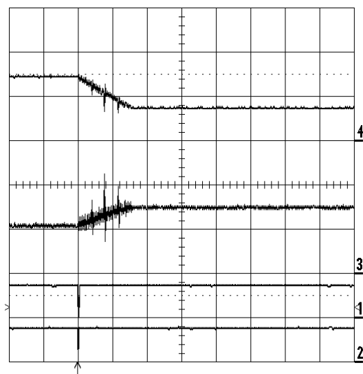
Waveform when it drives from code 256 to code 511 code 256
