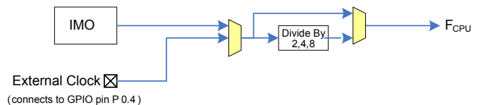
Figure 3. PSoC 4000 MCU Clocking Architecture
