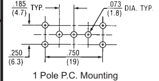
1 Pole P.C. Mounting
