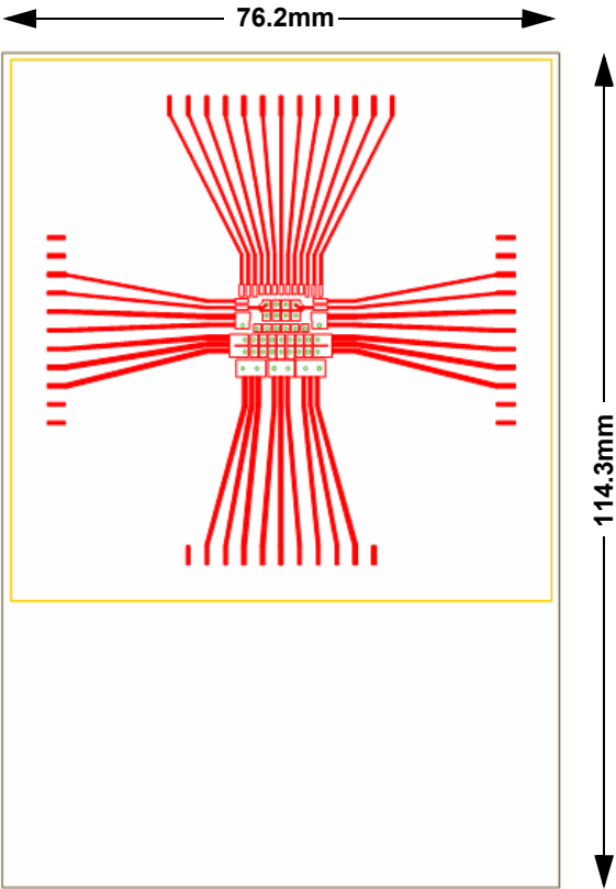
Figure 17. 2s2p JDEC Thermal Test Board (Red - Top Layer, Yellow - Two Buried Layers)
