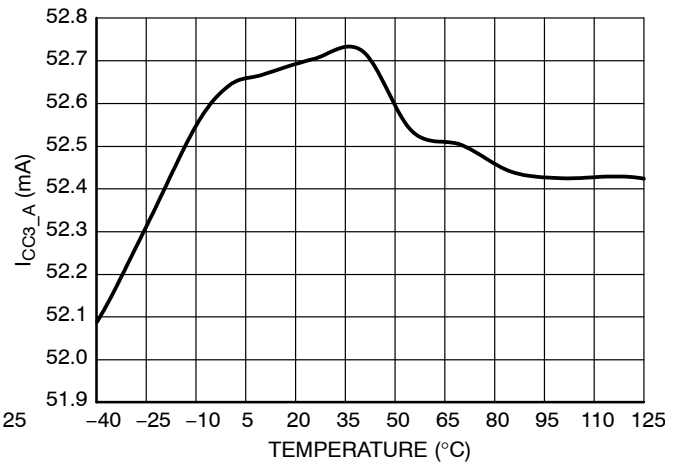
Figure 38. Internal IC Consumption (A Version, C DRV = 10 nF, f SW = 400 kHz, t on_min = 500 ns, t off_min = 620 ns)
