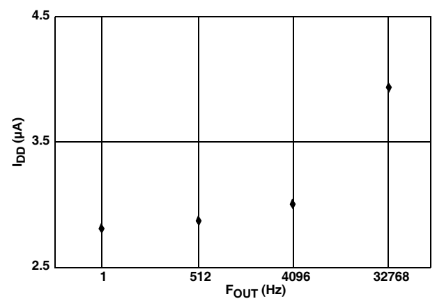
FIGURE 6. I DD1 vs f OUT AT V DD = 5V
