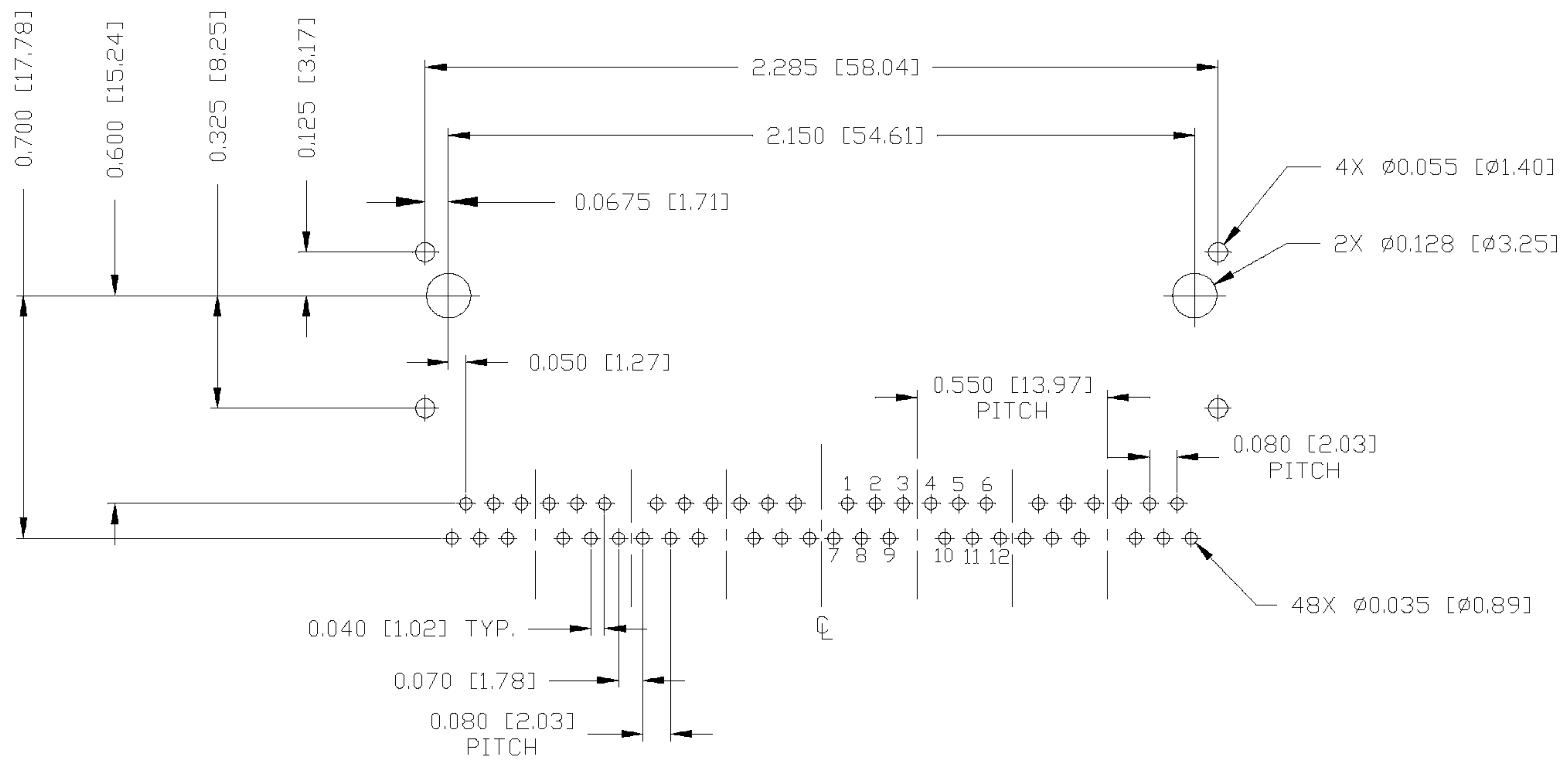
RECOMMENDED PCB FOOTPRINT COMPONENT SIDE VIEW
