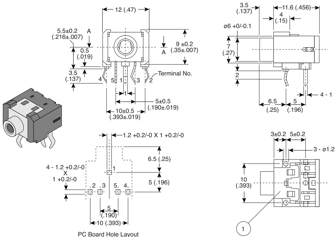
PC Board Hole Layout
