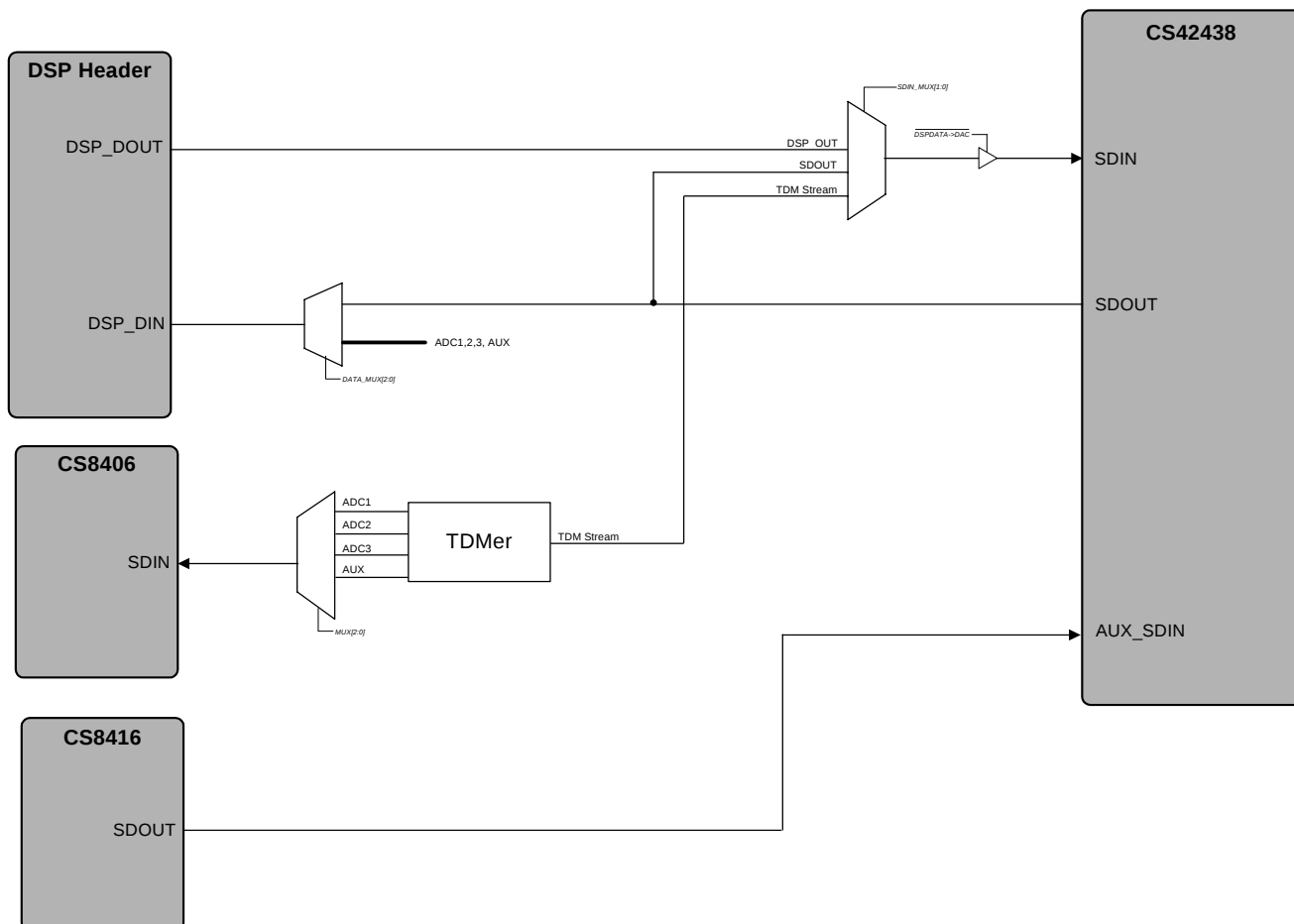
Figure 4. Internal Data Routing
