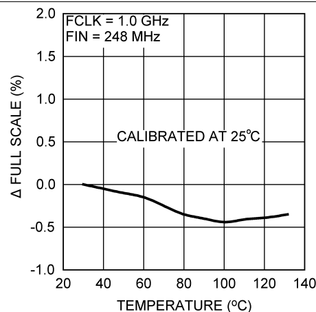
Figure 33. Gain vs Temperature FS Percent Change
