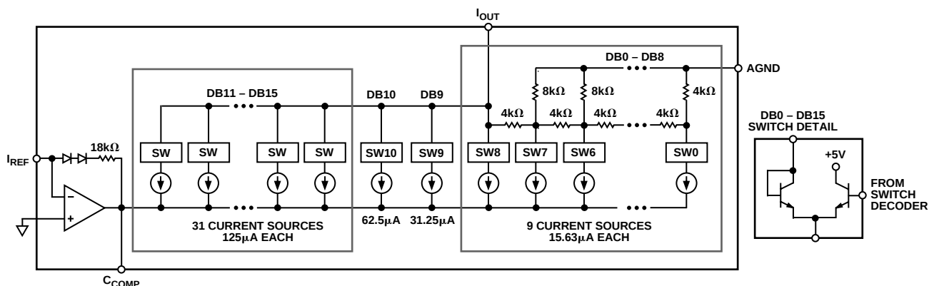
Figure 3. DAC16 Architecture
