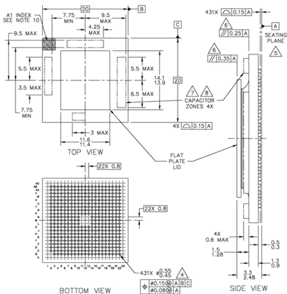
Figure 35. MSC8126 Mechanical Information, 431-pin FC-PBGA Package
