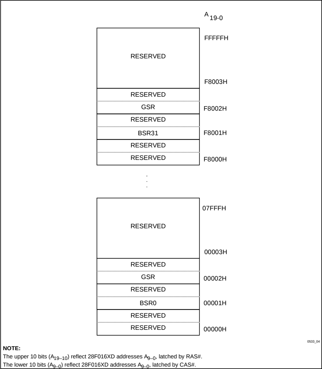
Figure 4. Extended Status Registers Memory Map
