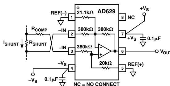
Figure 33. Compensating for Large Sense Resistors
