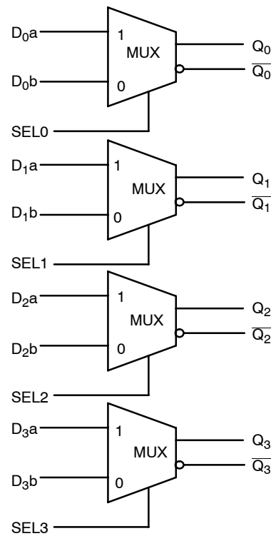
Figure 2. Logic Diagram
